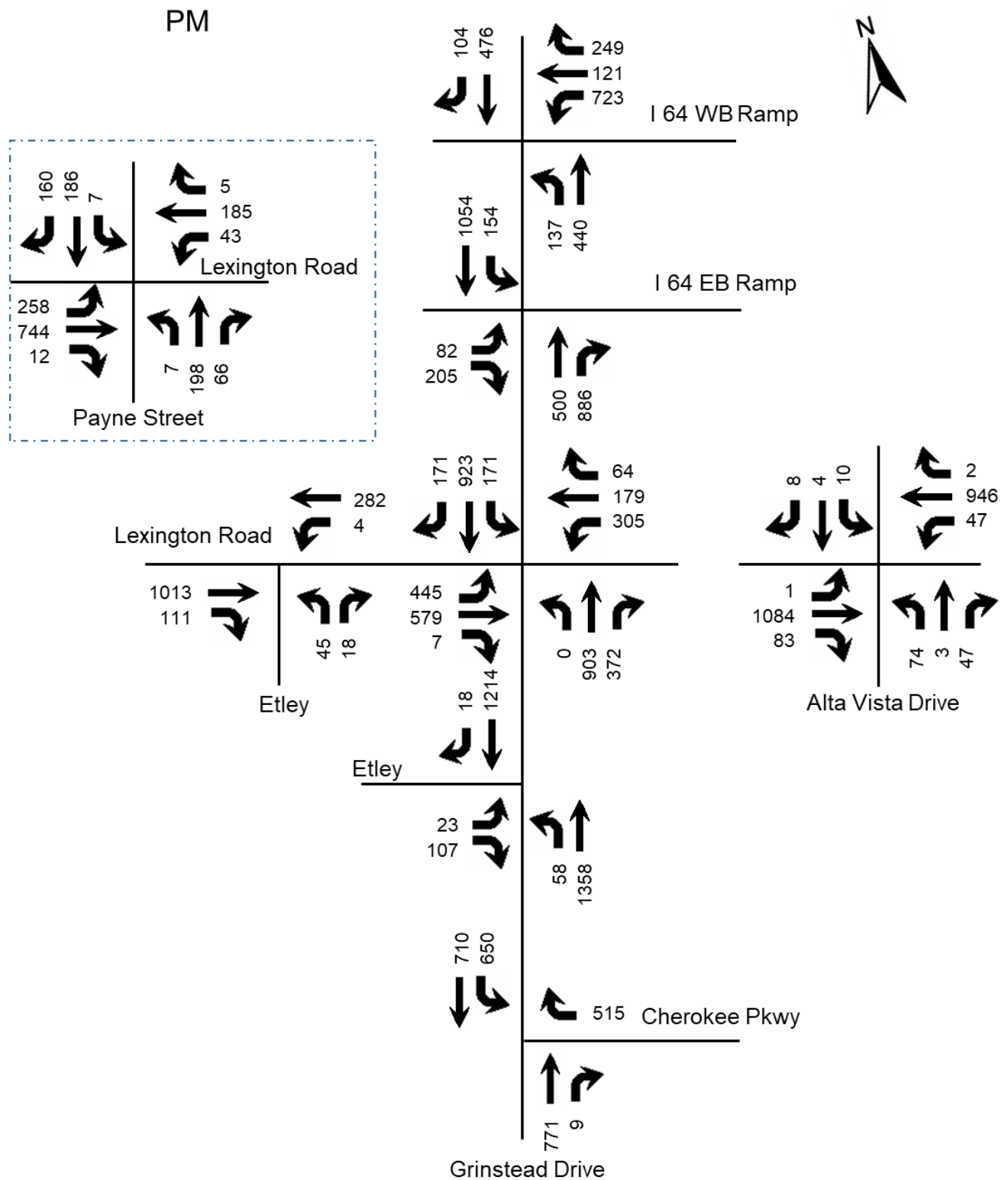
Figure 5. 2023 No Build PM Peak Hour Volumes
