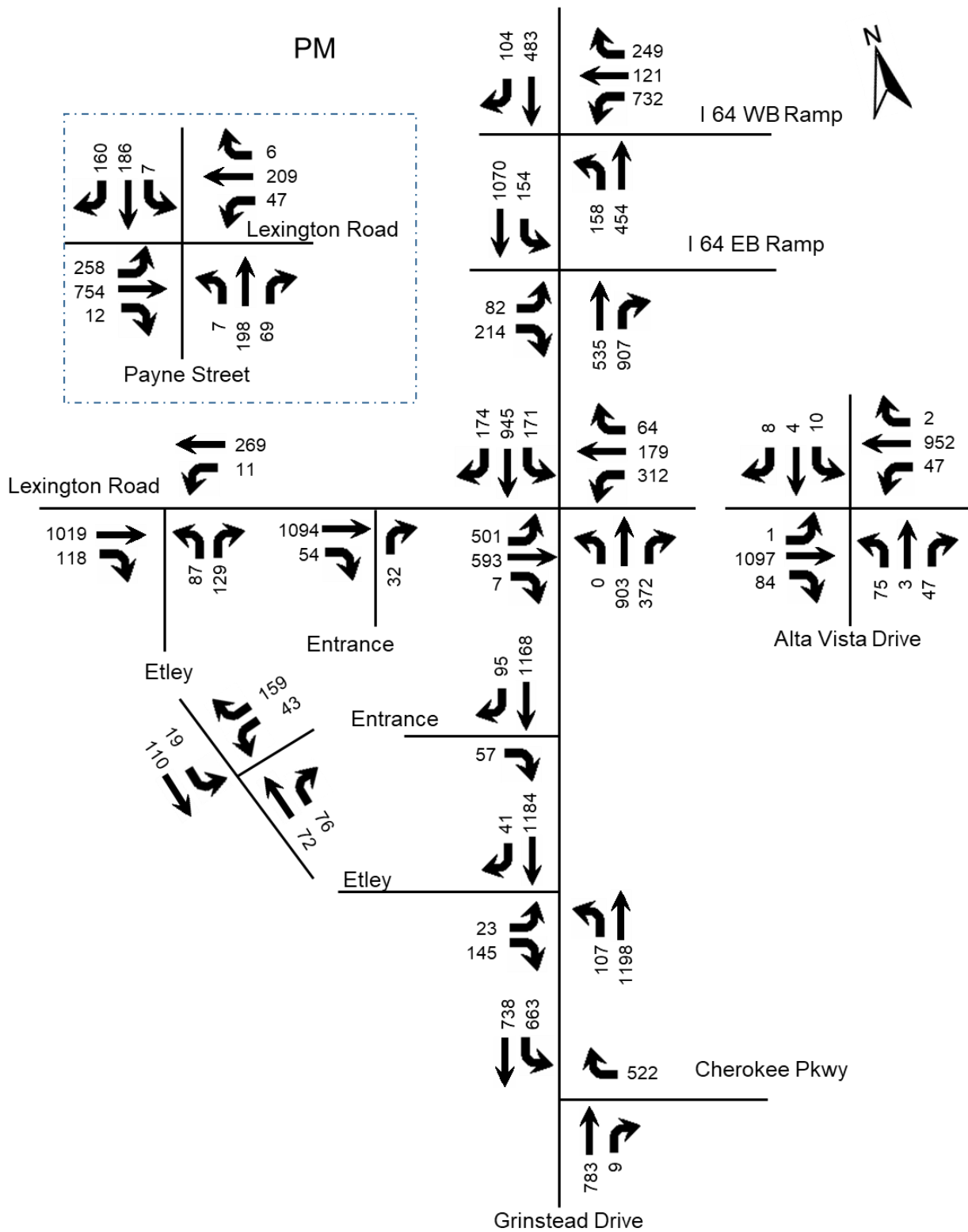
Figure 11. 2023 PM Peak Hour Build
