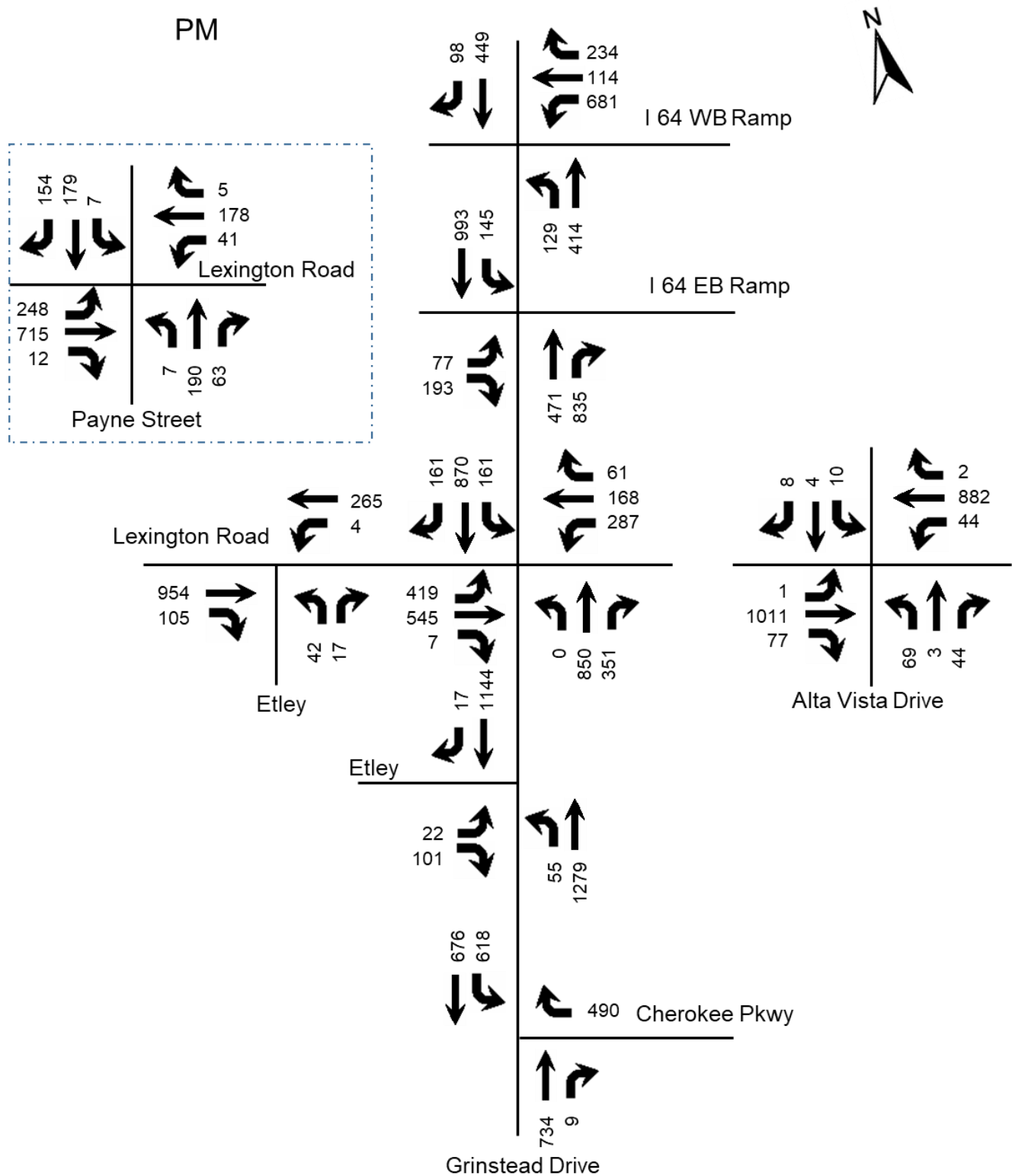
Figure 3. PM Existing Peak Hour Volumes
